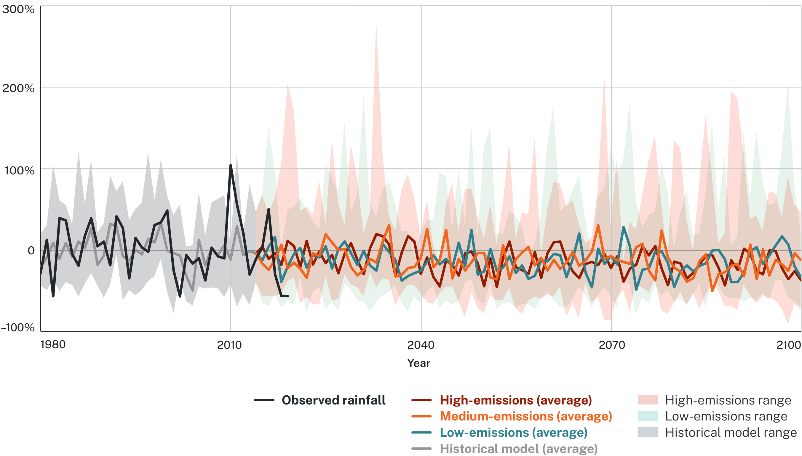
Figure 7. Historical and projected change in average rainfall – Far West
