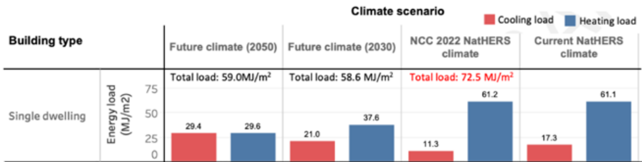
Figure 32: Comparing average heating, cooling loads of modified houses for the future climate (2050) with future (2030) and NatHERS climate files.
